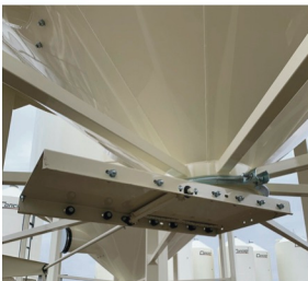
Adjustable Rack & Pinion Slide Gate Assembly. Available in Stainless Steel
